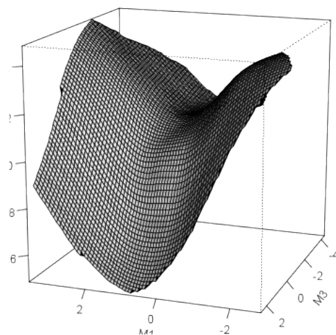
Fig. 1. The fitness surface of the m_1 and m_3 eigenvectors of the M matrix from the canonical analysis of y for the amino acid composition of the spermatophylax.
