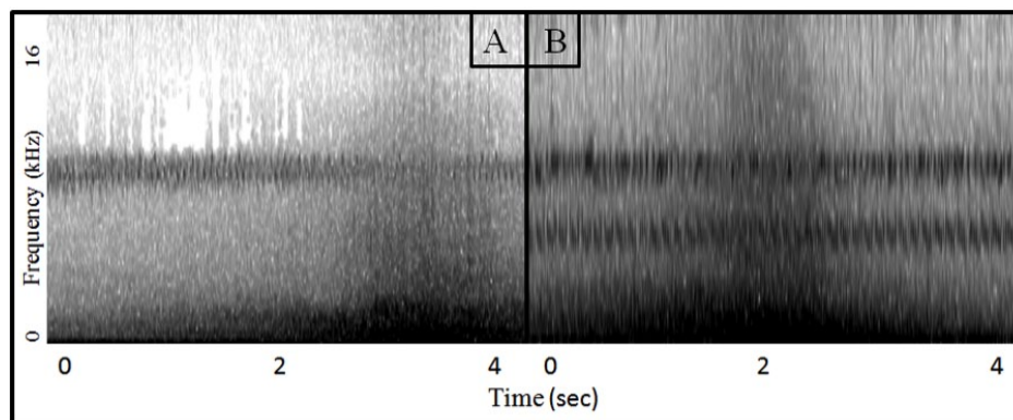
Fig. 1. Spectrogram of ambient noise 5-10 m from two roadsides in Hanover, New Hampshire. Sound profile includes of Allonemobius allardi (panel A and B, dominant frequency approx. 8 kHz) and Eunemobius carolina (panel B, dominant frequency approx. 5 kHz). Peak car noise occurs at approximately 3.5 seconds (panel A) and 2.0 seconds (panel B). Recording was generated using a Marantz 661 and an omnidirectional Sennheiser ME62 microphone positioned approximately 20 cm above ground level. The spectrogram was generated using RavenPro (Cornell Lab of Ornithology). Darker colors represent higher sound intensity.
